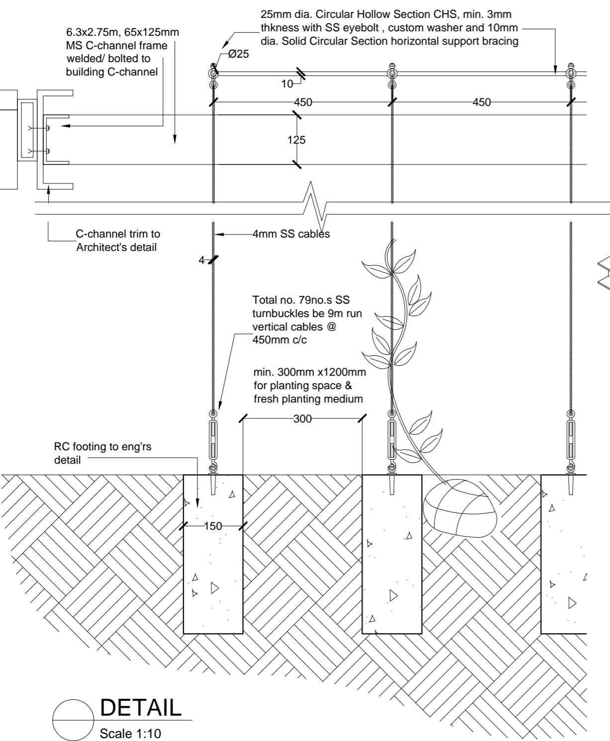
DETAIL Scale 1:10
