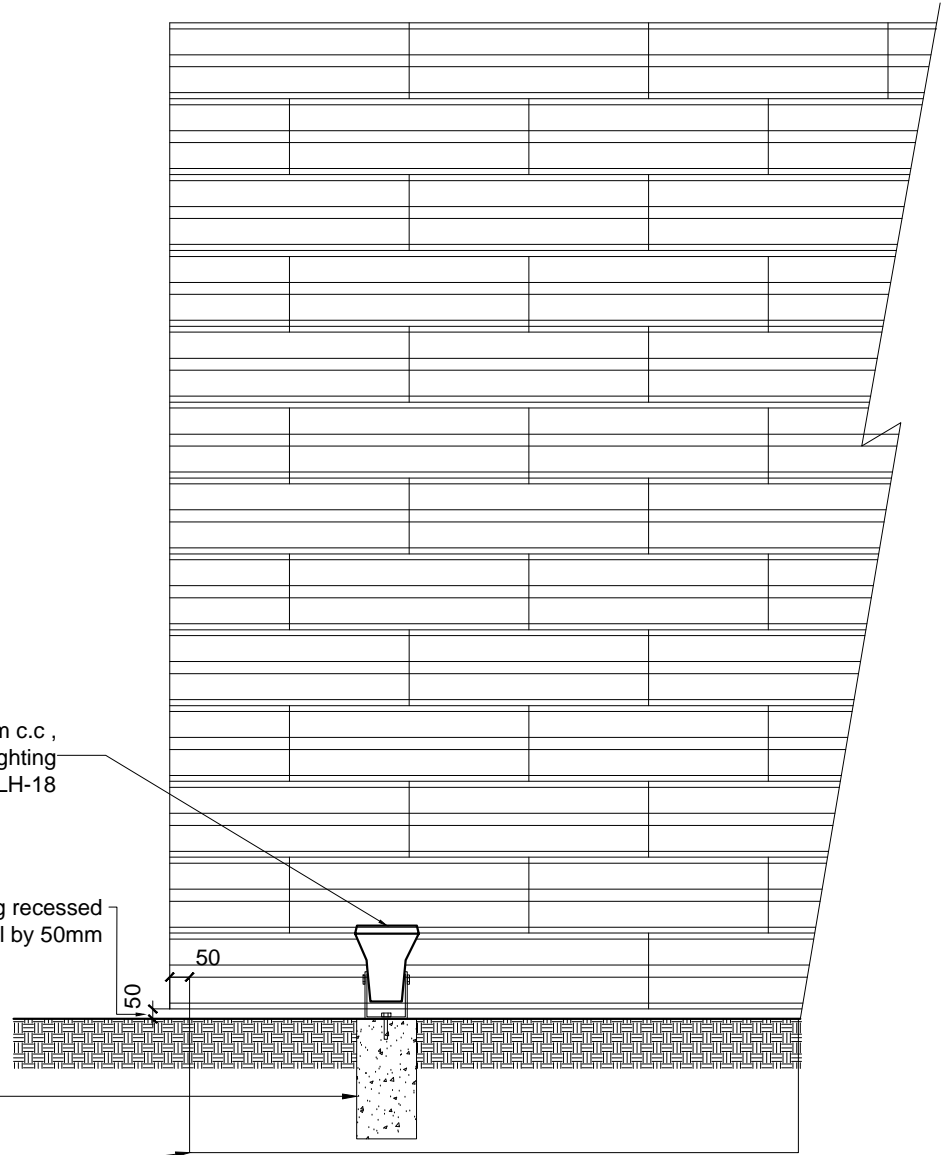
8a Typical Wall Elevation SCALE 1:20
