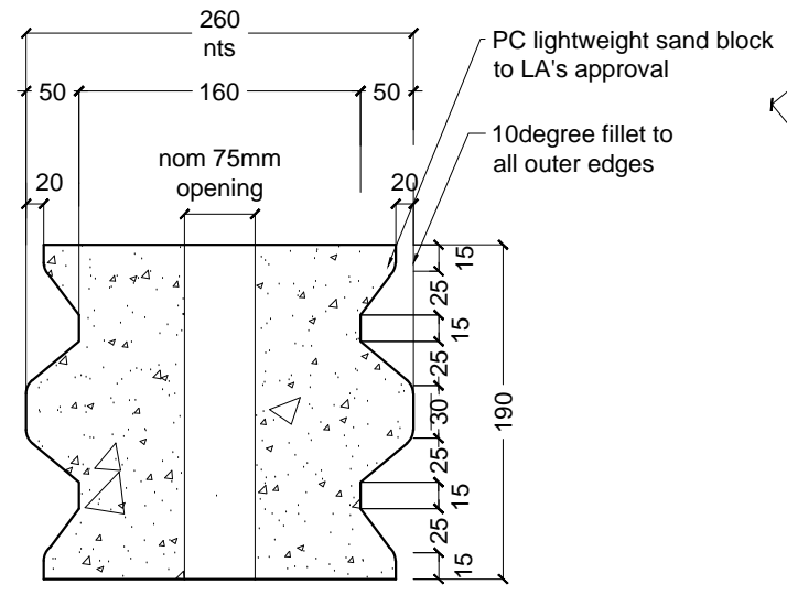
8b Typical Cement Block Section INSET SCALE 1:5
