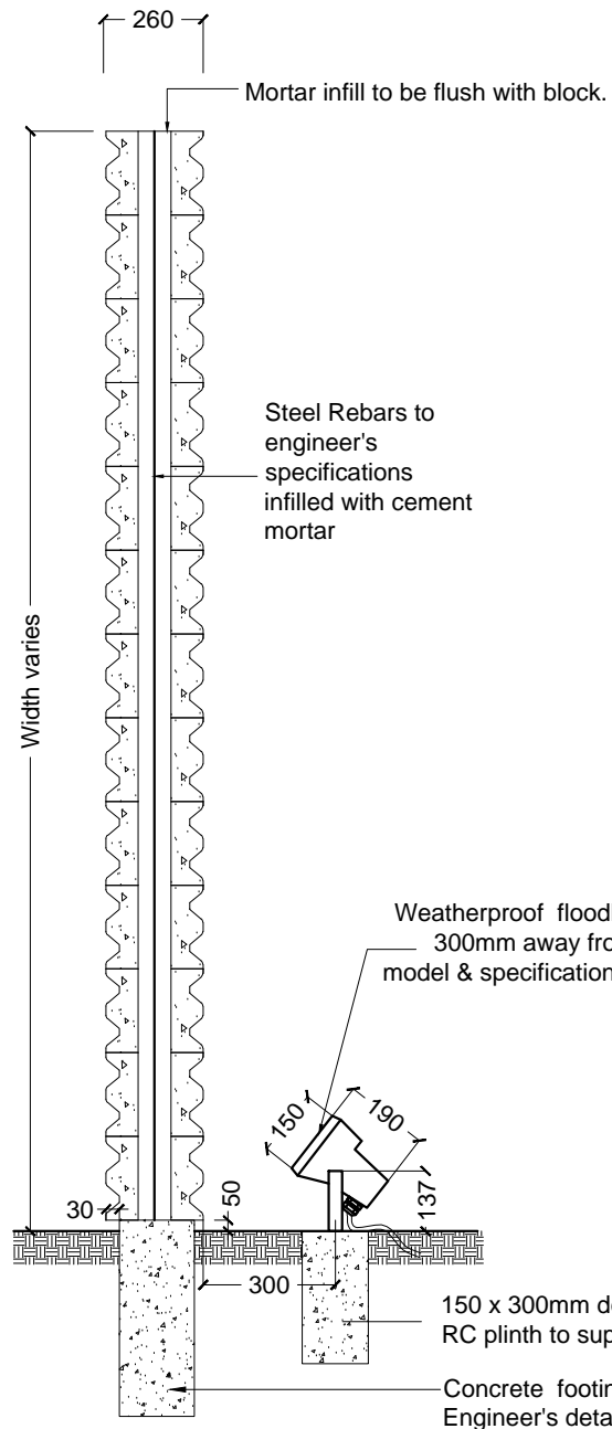
8 Typical Wall Section SCALE 1:20
