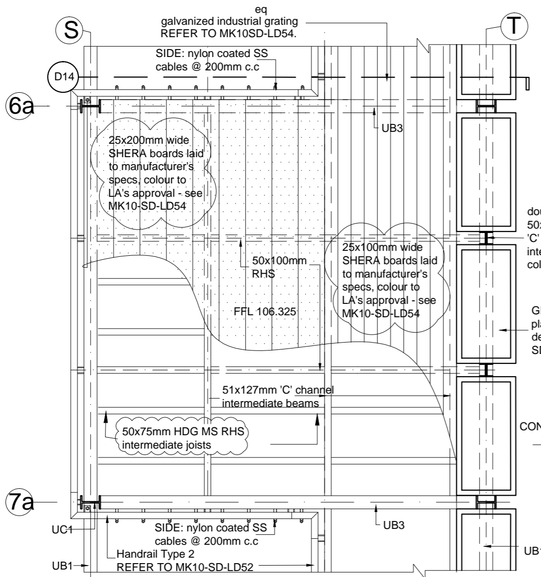
TYPICAL PLAN: Open Deck Type A (ODA) SCALE 1:30
