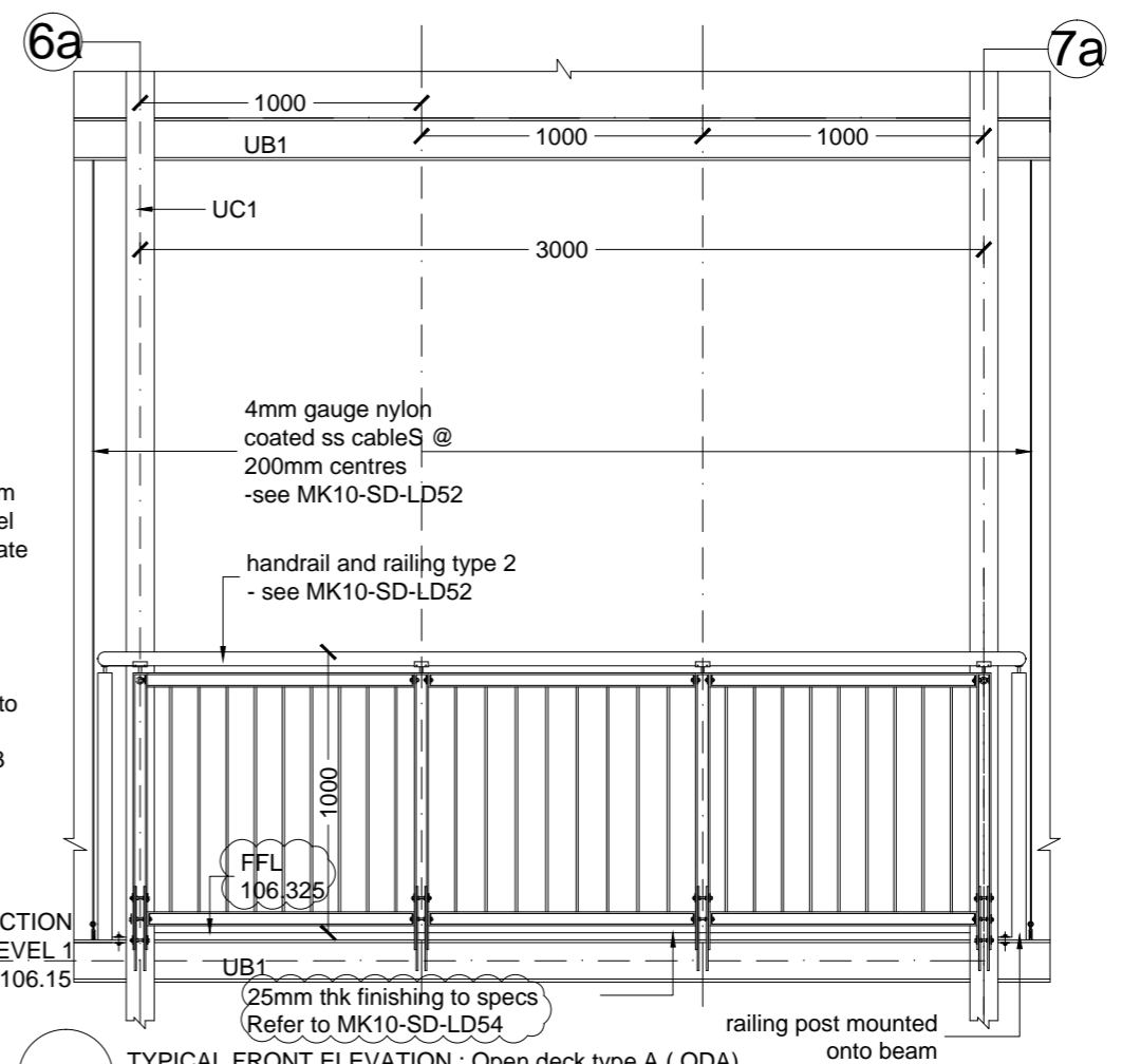
TYPICAL FRONT ELEVATION: Open deck type A ( ODA) SCALE 1:30
