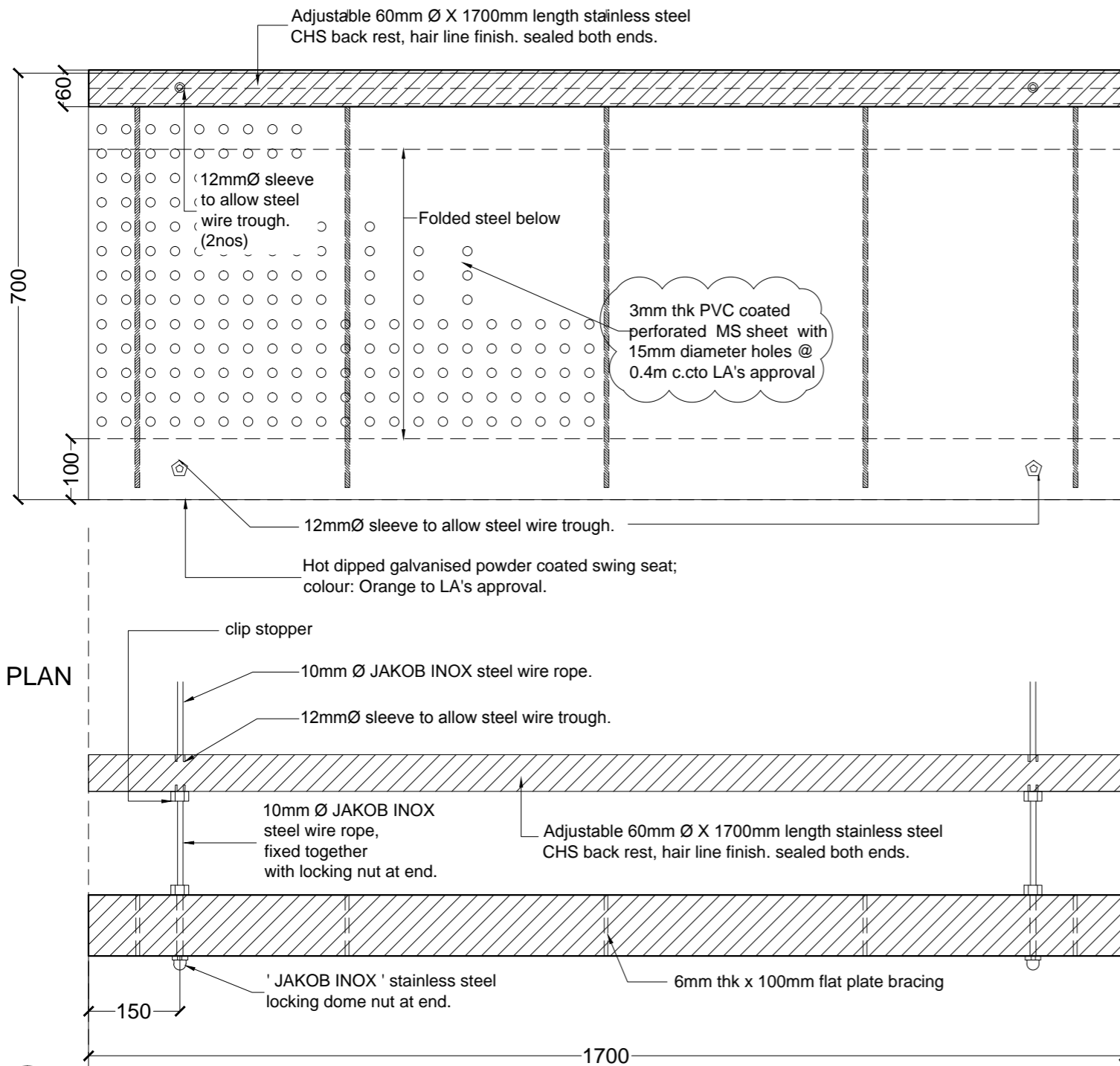
TYPICAL FRONT ELEVATION
