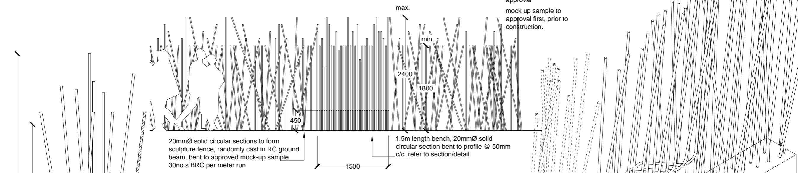
A SECTION : BRC fencing bench Scale 1:20
