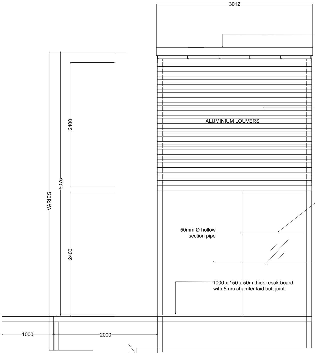
ELEVATION X Scale 1:40
