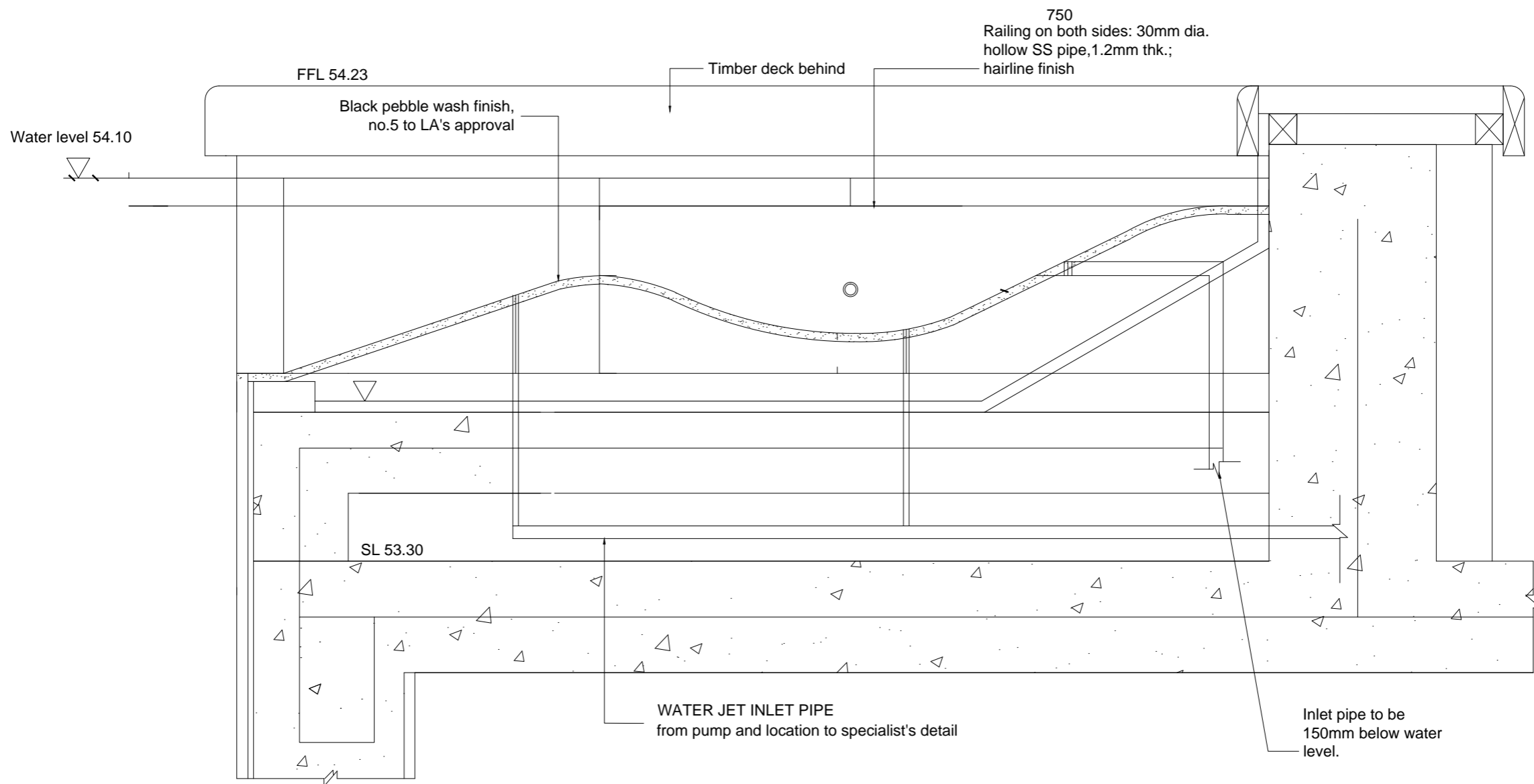
TYPICAL SECTION: Jacuzzi @ Lap Pool SCALE 1:10
